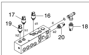
SHUTTLE BLOCK
